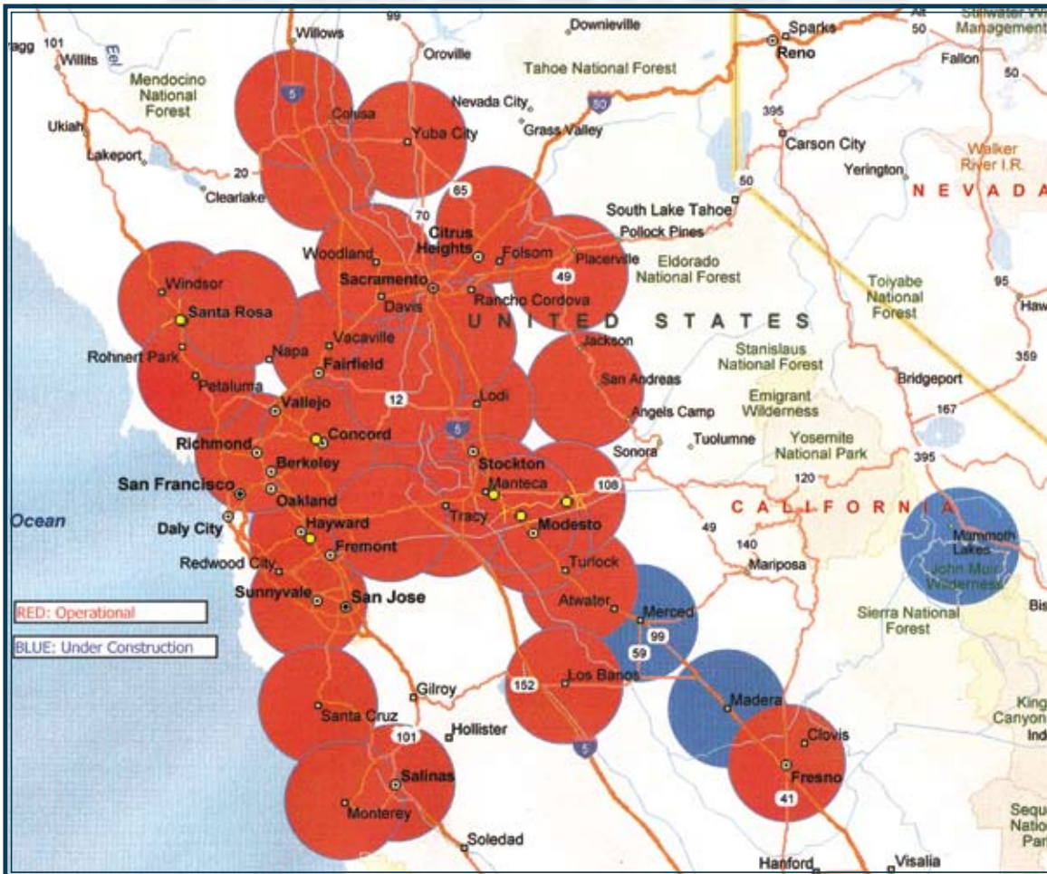
ESC RTK Reference Station Map As Of January 1, 2009
